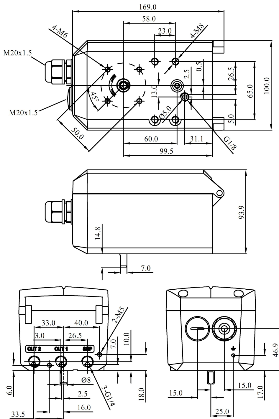
Positioner Dimensions
