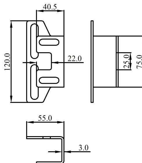
Remote linear mounting bracket
